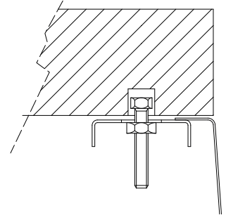
lateral section
